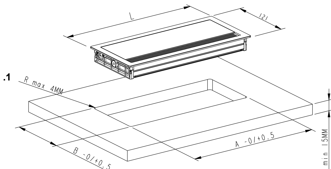
Fixing hole
